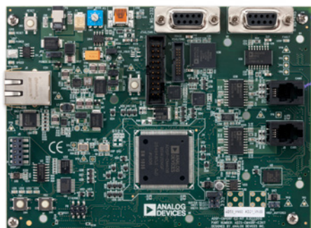
ADSP-CM408F motor drive control board (EZ-KIT®).
